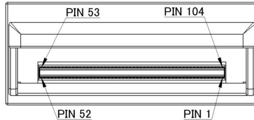
Figure2. Pad Layout of the CFP2 module
